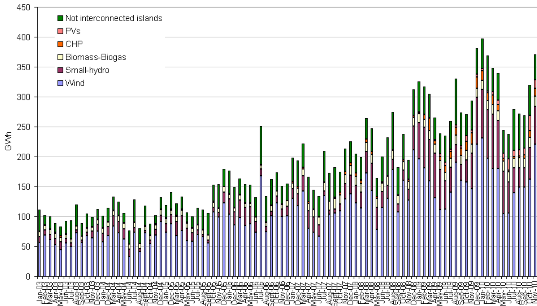
2003-2010 Total Greek electricity generation from RES and CHP (Art.9 and 10, Law 3468/2006)
