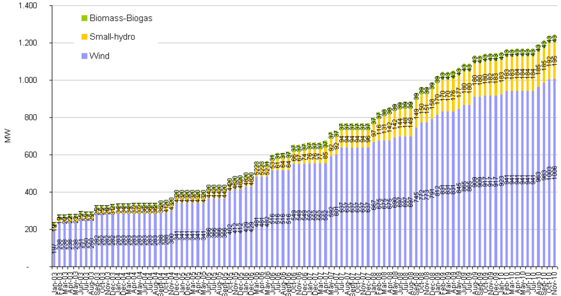
2003–2010 Installed RES capacity in the interconnected system (Art.9, Law 3468/2006)
